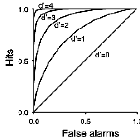
ROC curves
