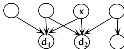
Figure 1: Whether independent data measures are singly connected to the estimated variable x determines whether or not estimation modules can be created for x .
