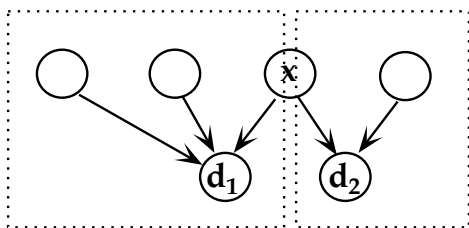
Figure 1: Whether independent data measures are singly connected to the estimated variable x determines whether or not estimation modules can be created for x .
